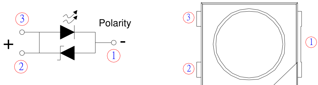
< Figure 2 PLCC 3528 series circuit diagram >
