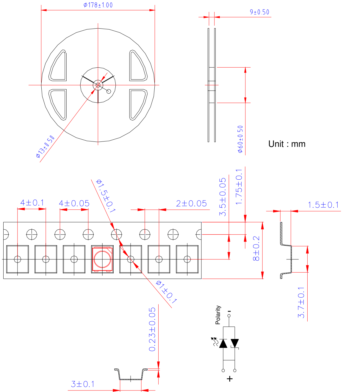
< Figure 9 Taping reel dimensions >
