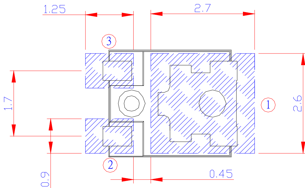
<Figure 7 Pad Dimension >
