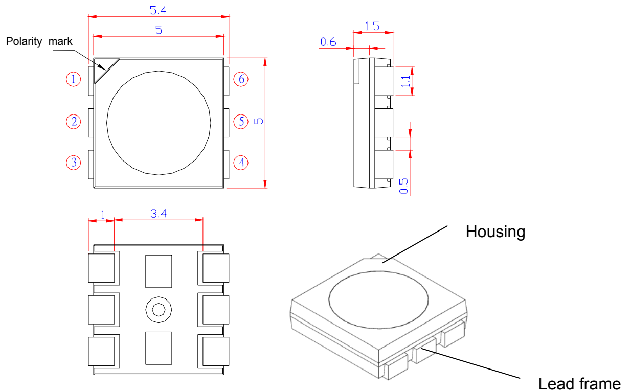
< Figure 1 PLCC 5050 series dimensions >
