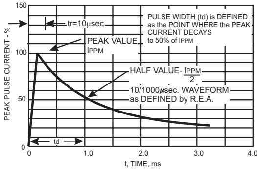
FIG.3- PULSE WAVEFORM
