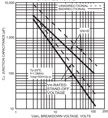
FIG.5- TYPICAL JUNCTION CAPACITANCE UNIDIRECTIONAL
